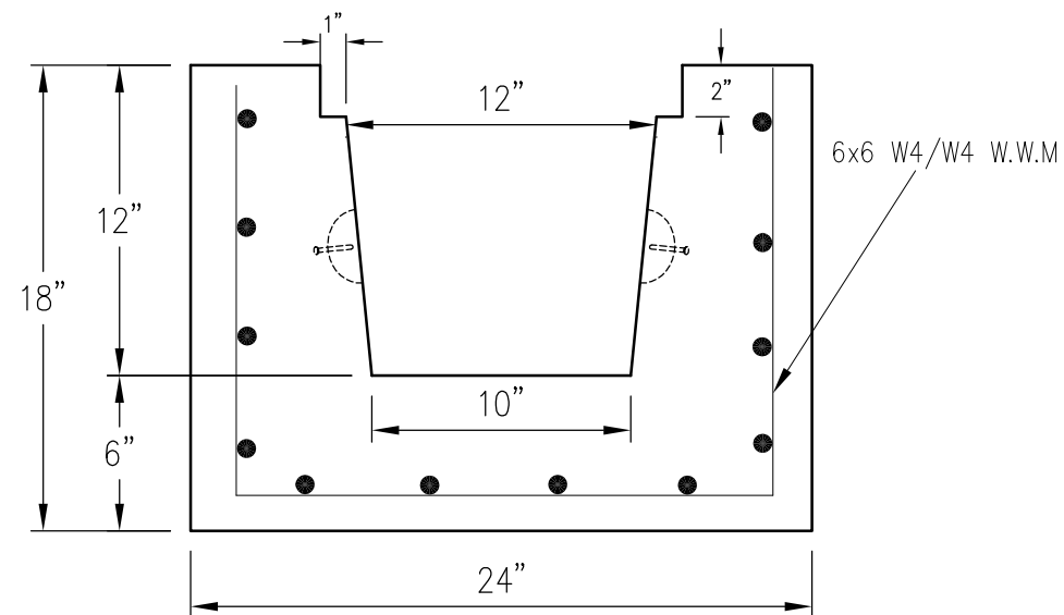
TRENCH DETAIL
