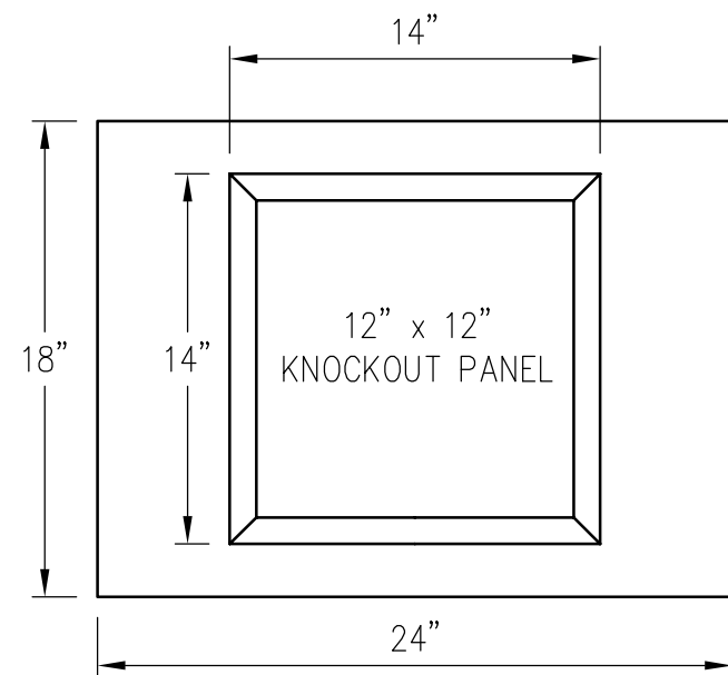
KNOCKOUT DETAIL
