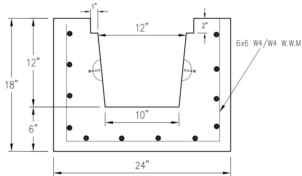
TRENCH DETAIL
