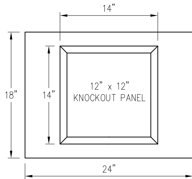
KNOCKOUT DETAIL
