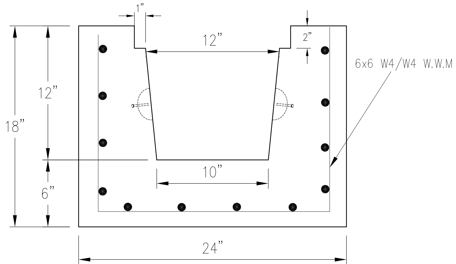
TRENCH DETAIL
