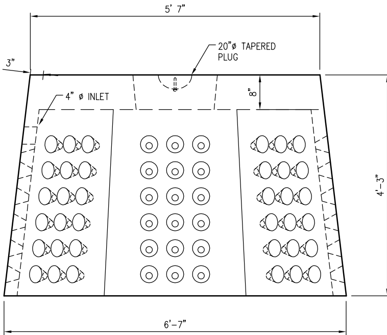
ELEVATION VIEW SCALE: 1/2" = 1'-0"
