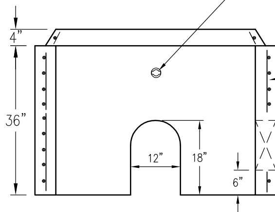
SECTION VIEW
