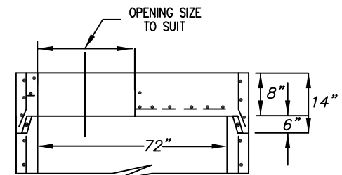
TYPICAL 72" DIA MANHOLE WITH TOP SLAB *BUTT JOINT OPTION ALSO AVAILABLE
