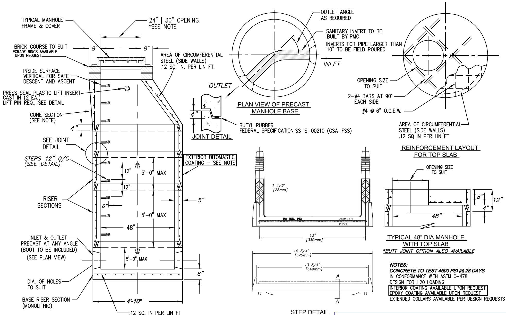
MANHOLE ASSEMBLY
