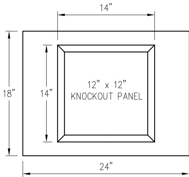
KNOCKOUT DETAIL
