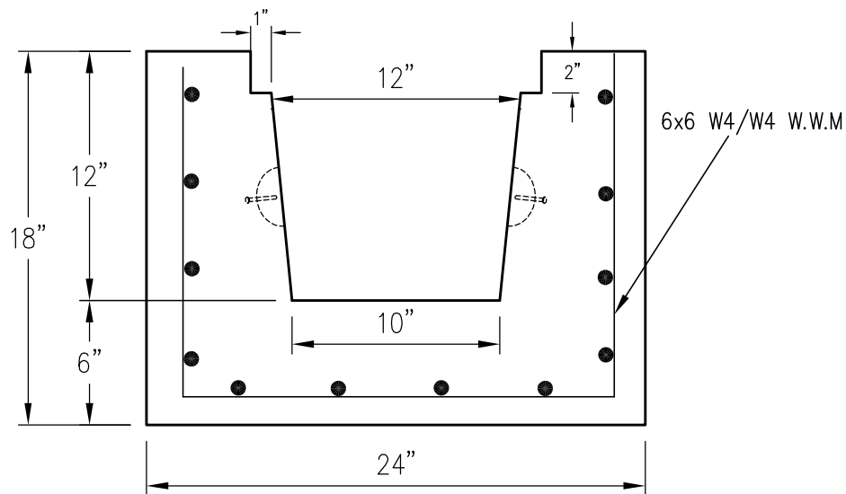
TRENCH DETAIL
