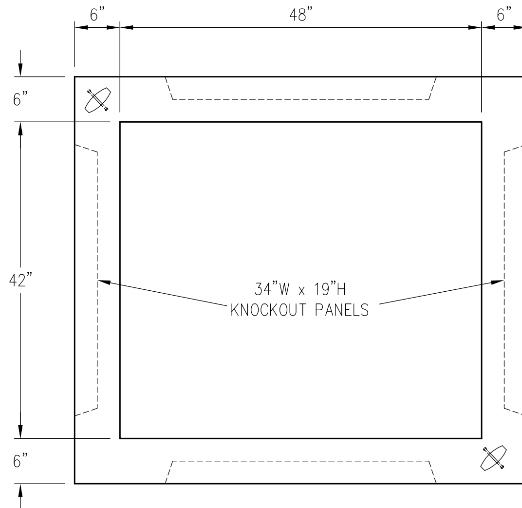
PLAN VIEW
