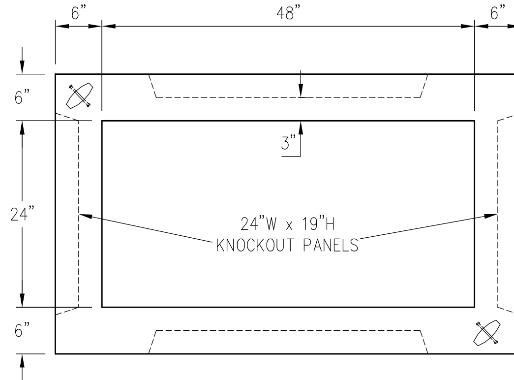
PLAN VIEW
