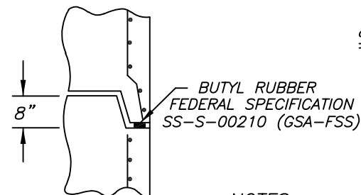
JOINT DETAIL
