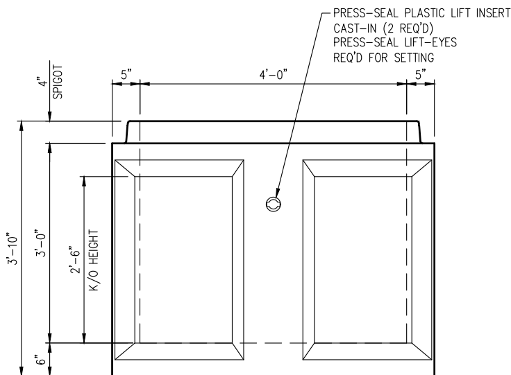
ELEVATION VIEW
