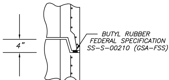
JOINT DETAIL
