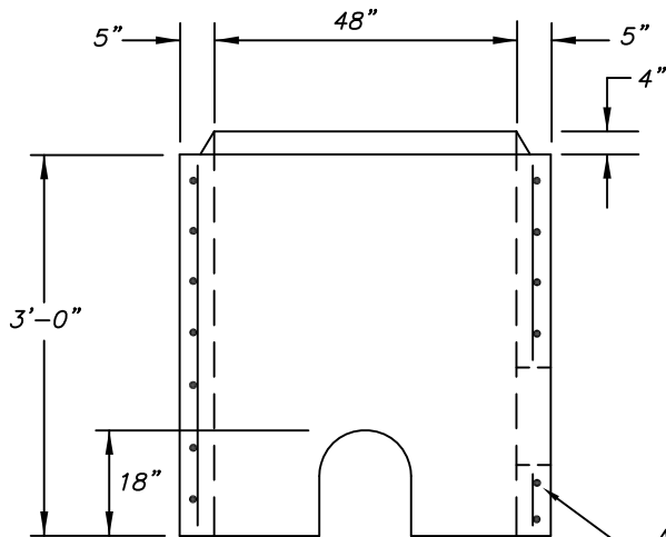
BARREL ELEVATION
