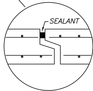
JOINT DETAIL
